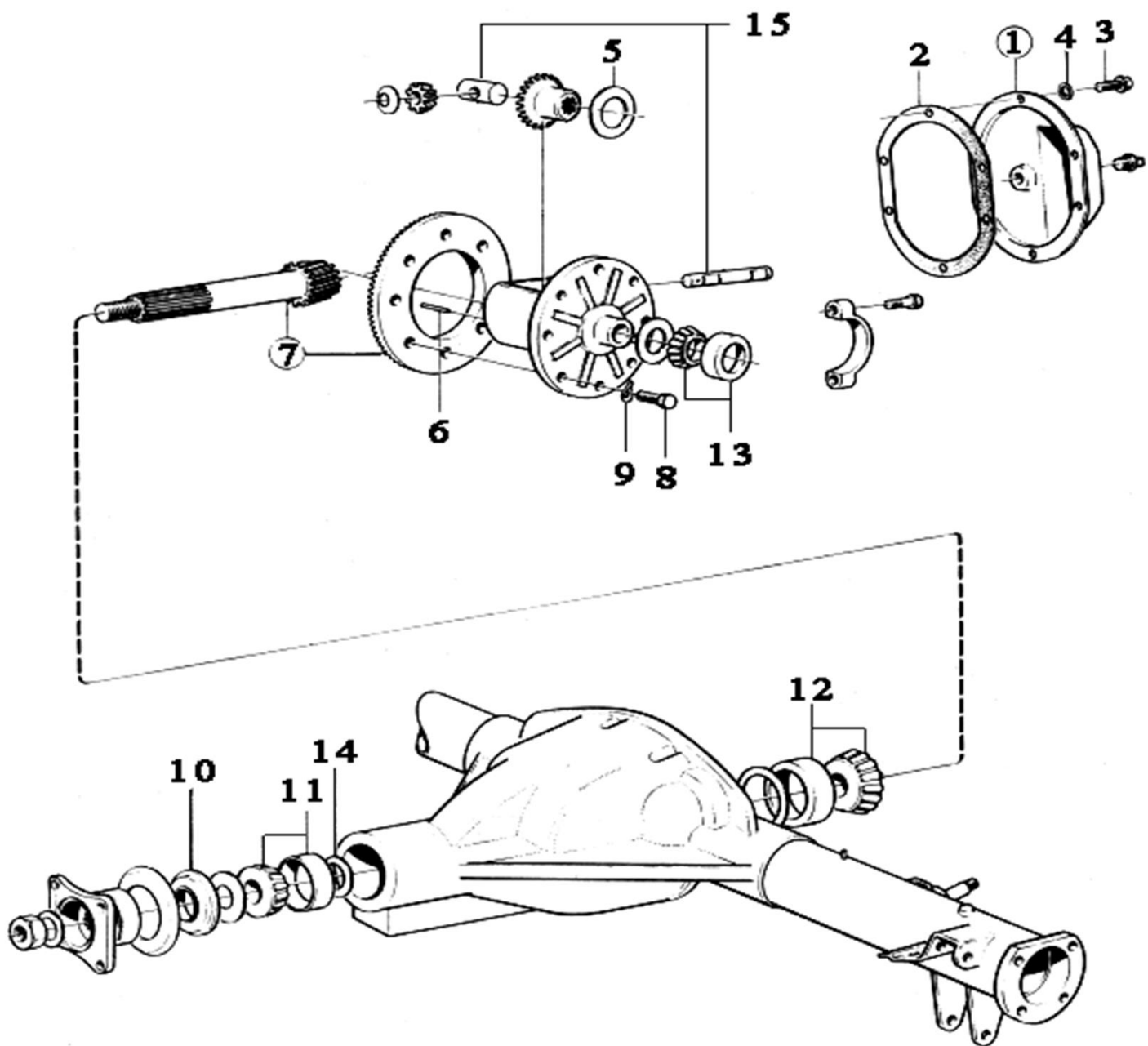
Fig. 4 Rear axle (67-72)
