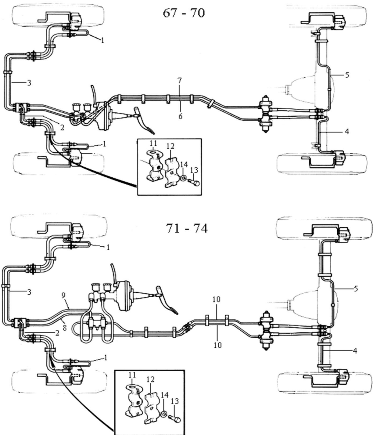
Fig 6: Brakelining
