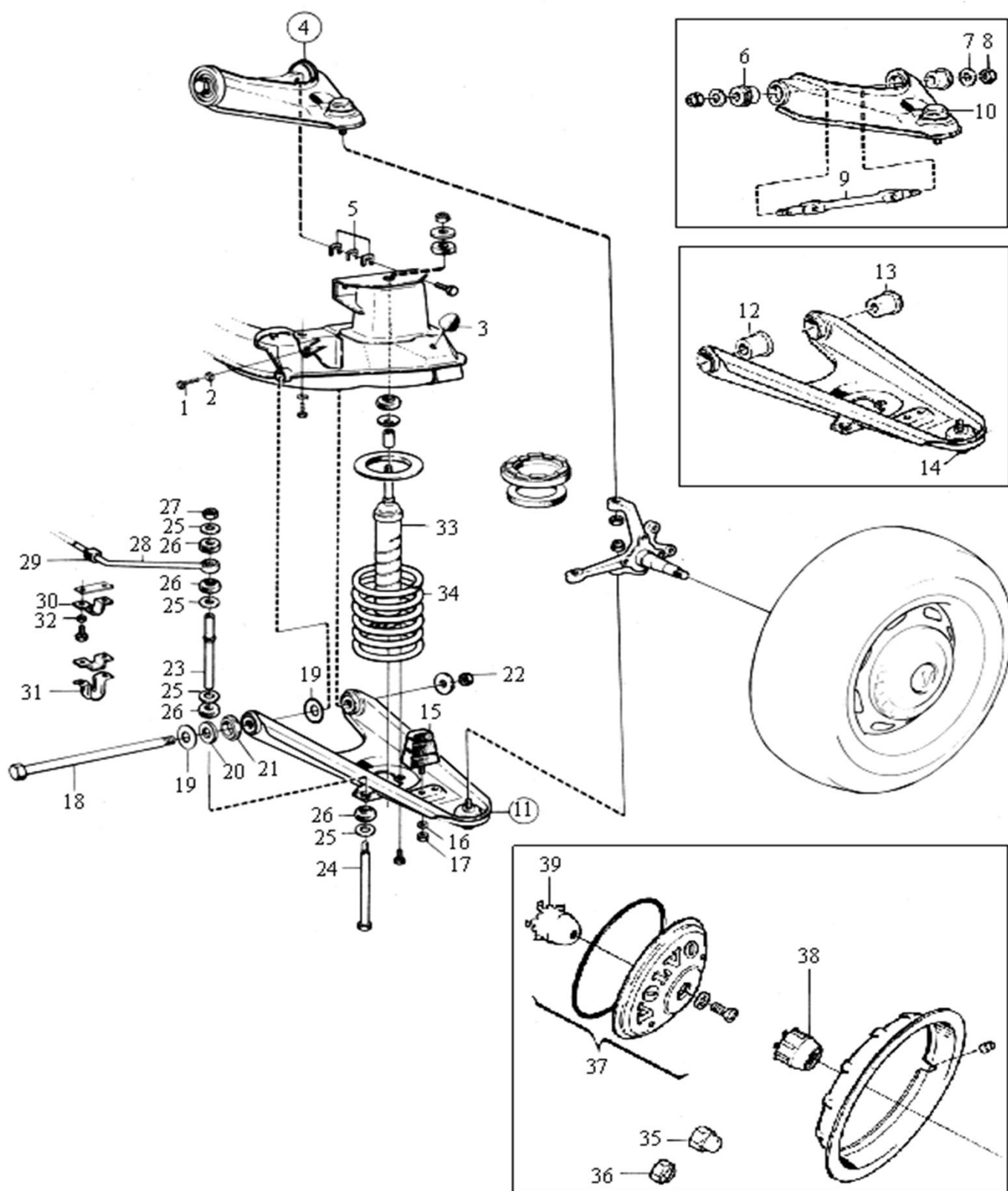
Fig. 2: Front suspension 140 (67-72)
