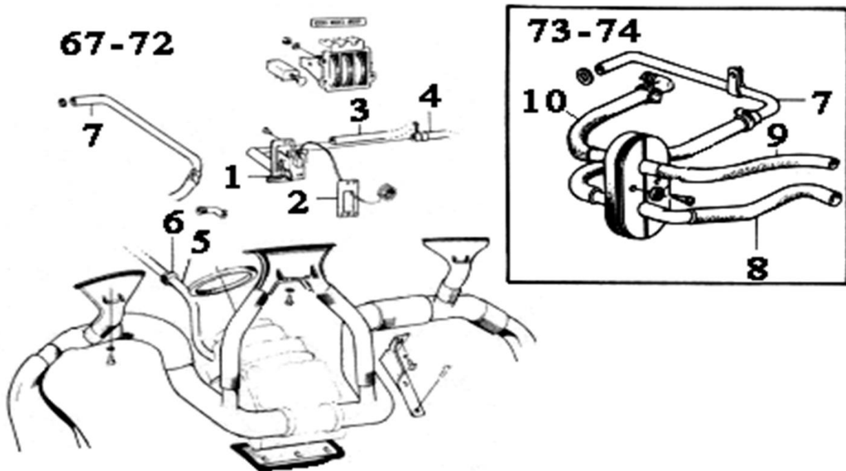
Fig. 1: Heater system 140
