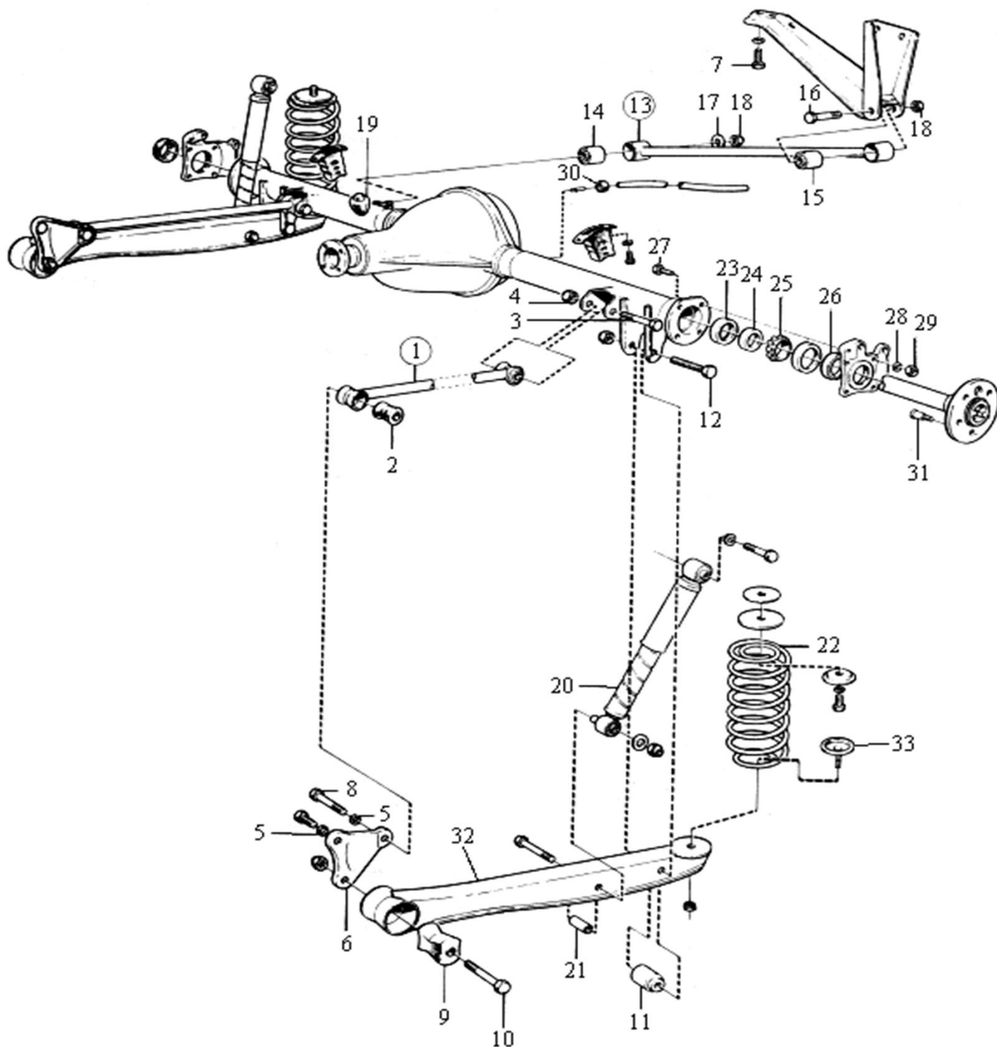
Fig 3: Parts for Rear Axle Mountings (67-72)
